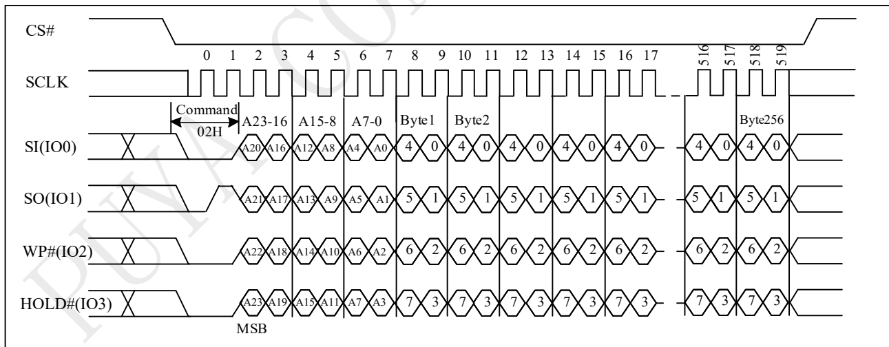
Figure 10-26a Page Program (PP) Sequence (QPI)
