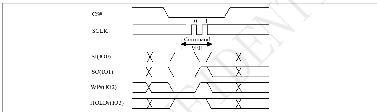
Figure 10-28a Buffer Clear Sequence (QPI)
