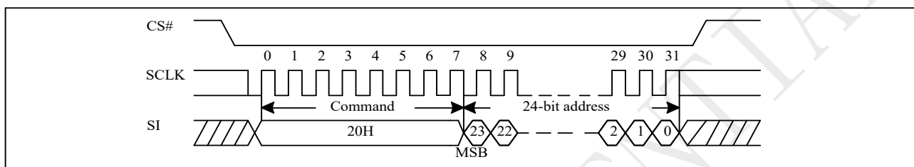
Figure 10-22 Sector Erase (SE) Sequence (Command 20)
