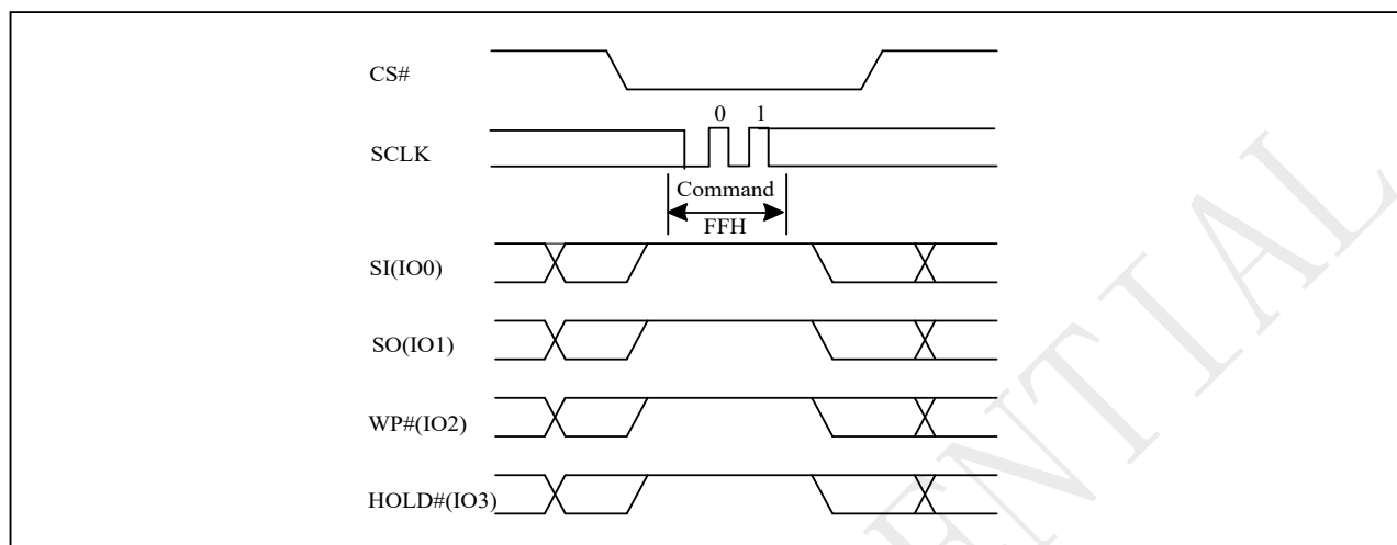
Figure 10-20 Disable QPI Sequence (QPI)
